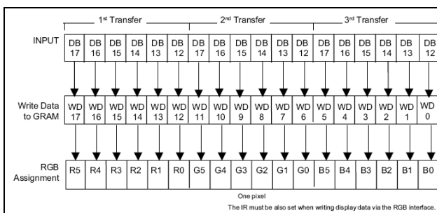
Figure 6-18 6-bit RGB interface (262,144 colors)
