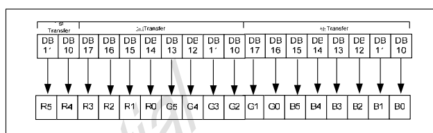
Figure 6-14 8-bit interface (262 colors) TRIREG = 1, DFM=0.
