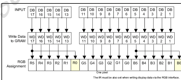
Figure 6-17 16-bit RGB interface (65,563 colors)
