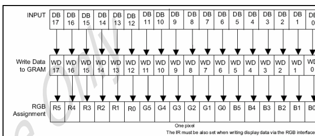
Figure 6-16 18-bit RGB interface (262,144 colors)
