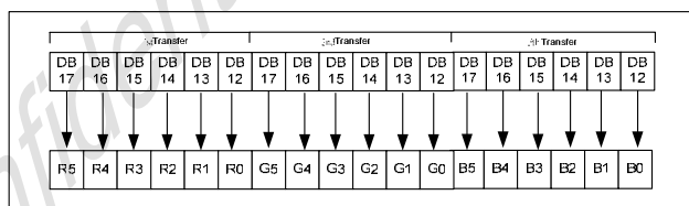
Figure 6-15 8-bit interface (262K colors) TRIREG = 1, DFM=1
