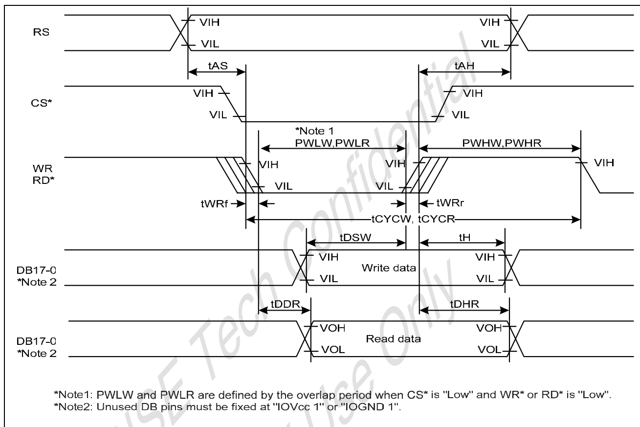
80-System Bus Interface
